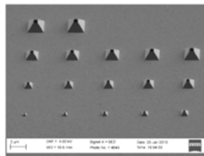
Fig. 2: SEM image: View angle of 45°, thin gold layer tipless pyramids, base lengths from 0.5 to 2.1 µm. Aperture sizes from 125 to 510 nm.
